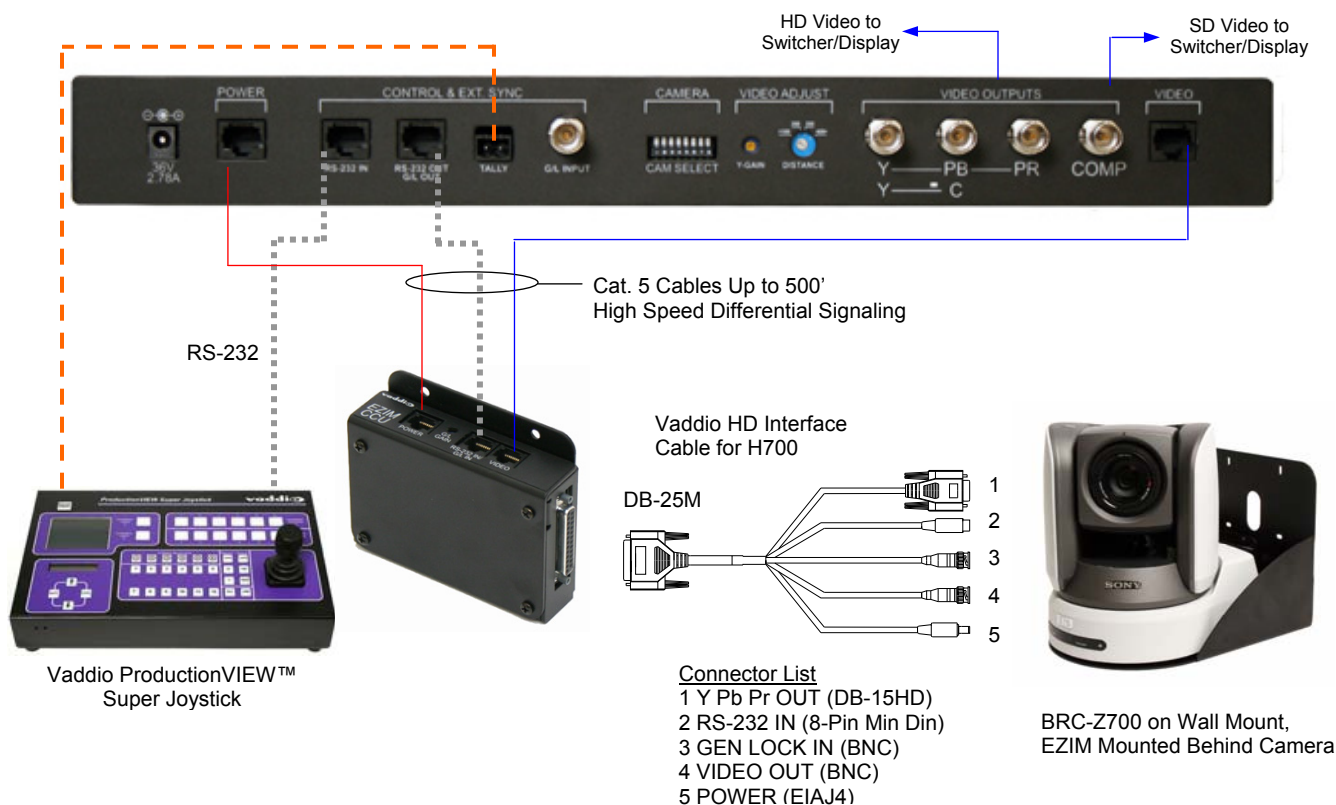
Figure 4: Basic system connectivity of a WallVIEW CCU Z700 System and ProductionVIEW Super Joystick Controller
